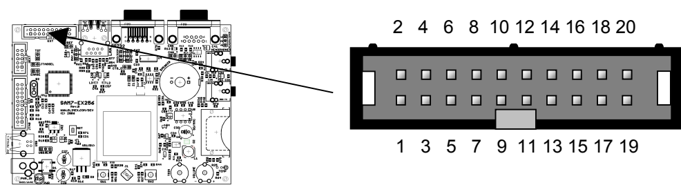
Figure 9-13 - EXT Connector
