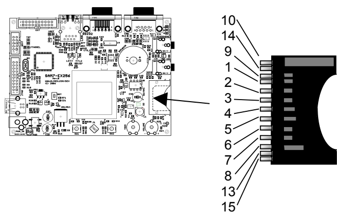
Figure 9-8 - SD/MMC Connector
