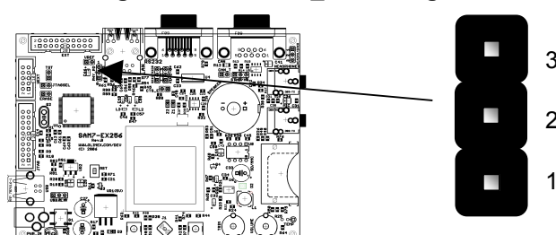
Figure 10-17 – PHY_PD Configuration
