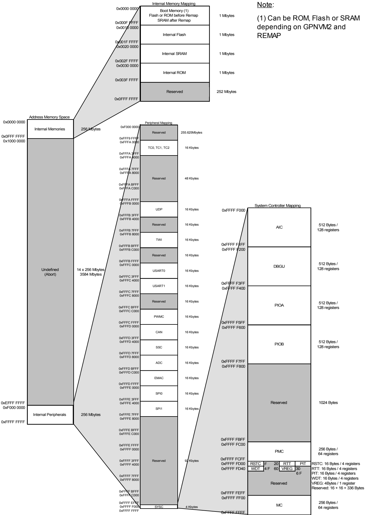
Figure 11-28 - Memory Map
