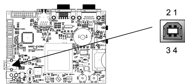
Figure 9-7 - USB Connector
