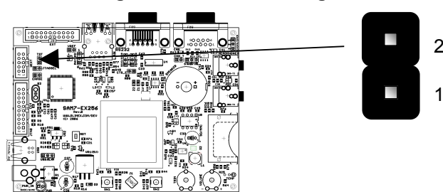
Figure 10-27 - TST Configuration
