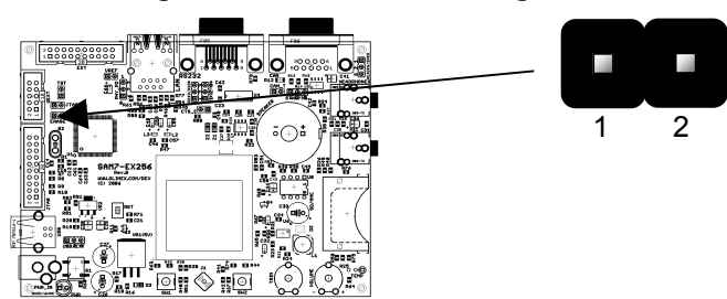
Figure 10-26 - ERASE Configuration
