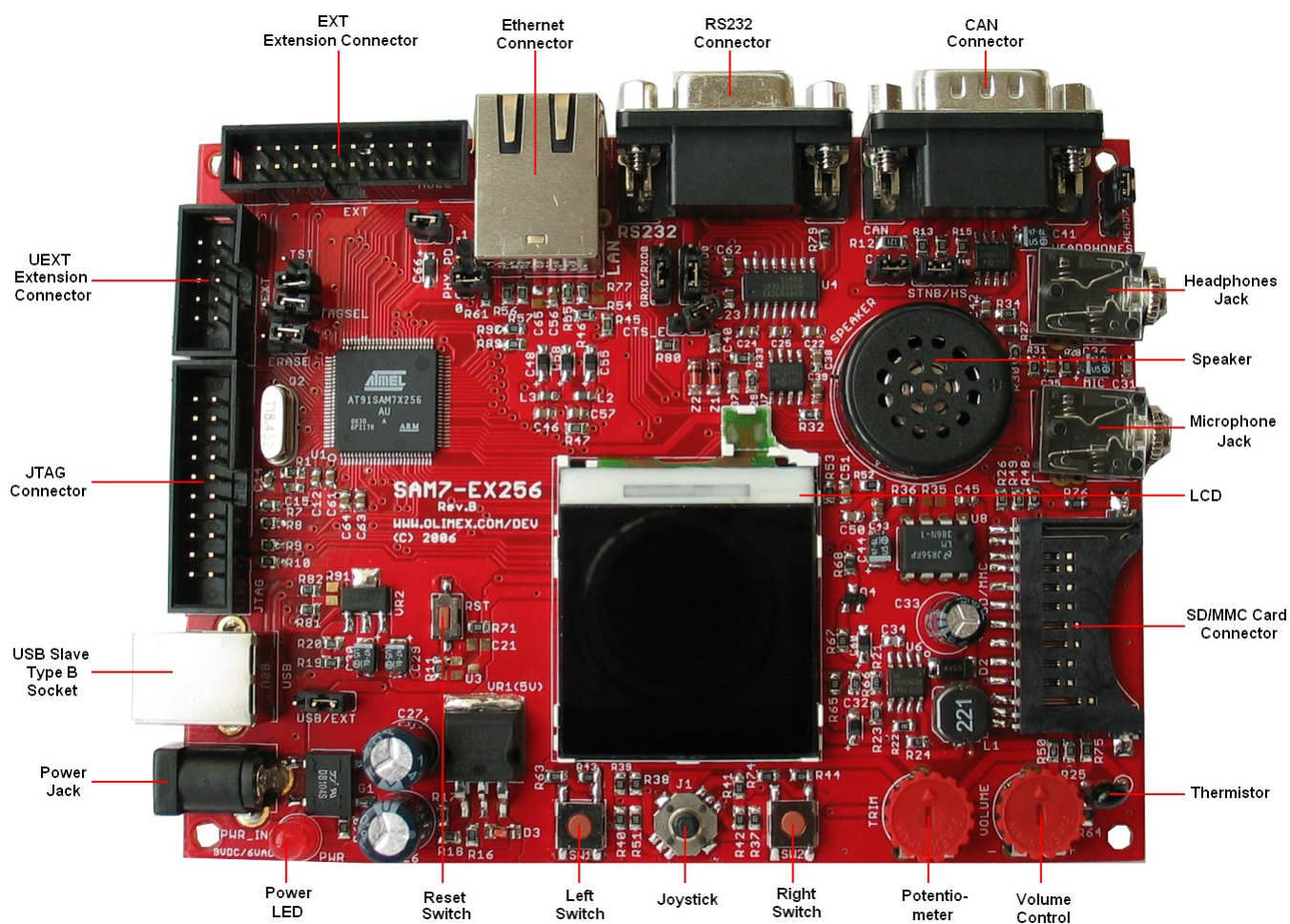
Figure 3-2. Board Layout
