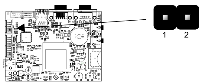
Figure 10-25 - JTAGSEL Configuration
