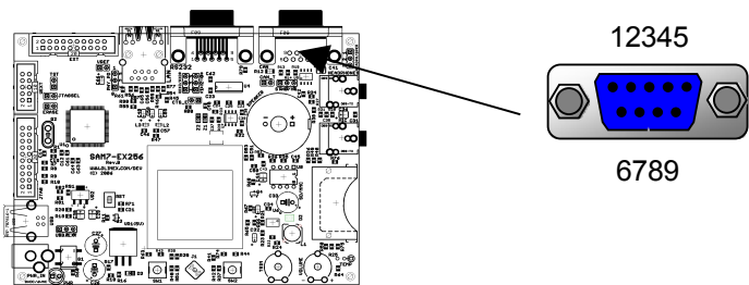
Figure 9-10 - CAN Bus Connector
