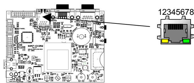
Figure 9-6 - Ethernet Connector
