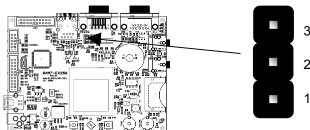
Figure 10-18 - DRXD/RXD0 Configuration
