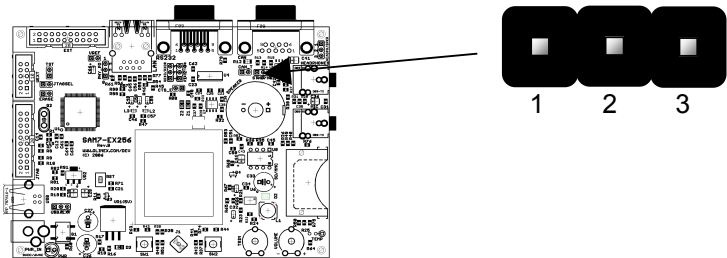
Figure 10-21 - STNB/HS Configuration
