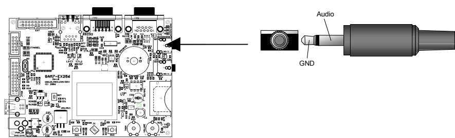
Figure 9-12 - Headphone Connector
