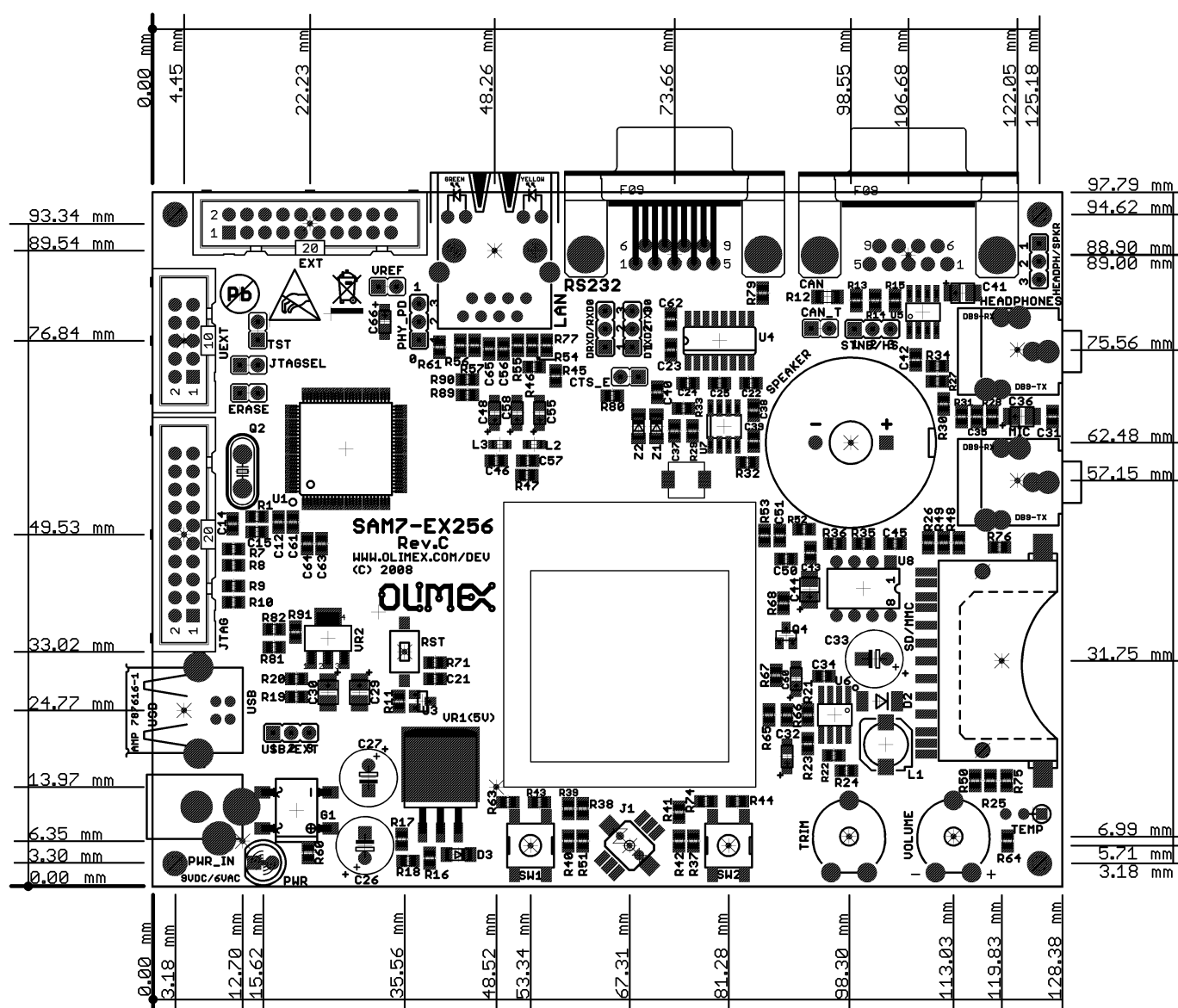
Figure 13-30. Mechanical Drawing
