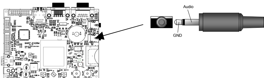
Figure 9-11 - Microphone Connector
