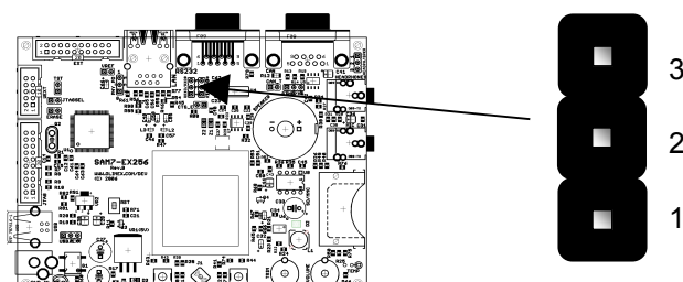
Figure 10-19 - DTXD/TXD0 Configuration
