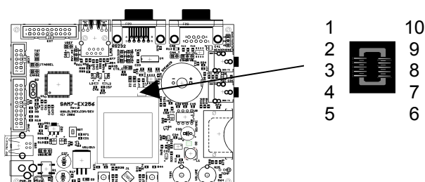
Figure 9-5 - LCD Connector
