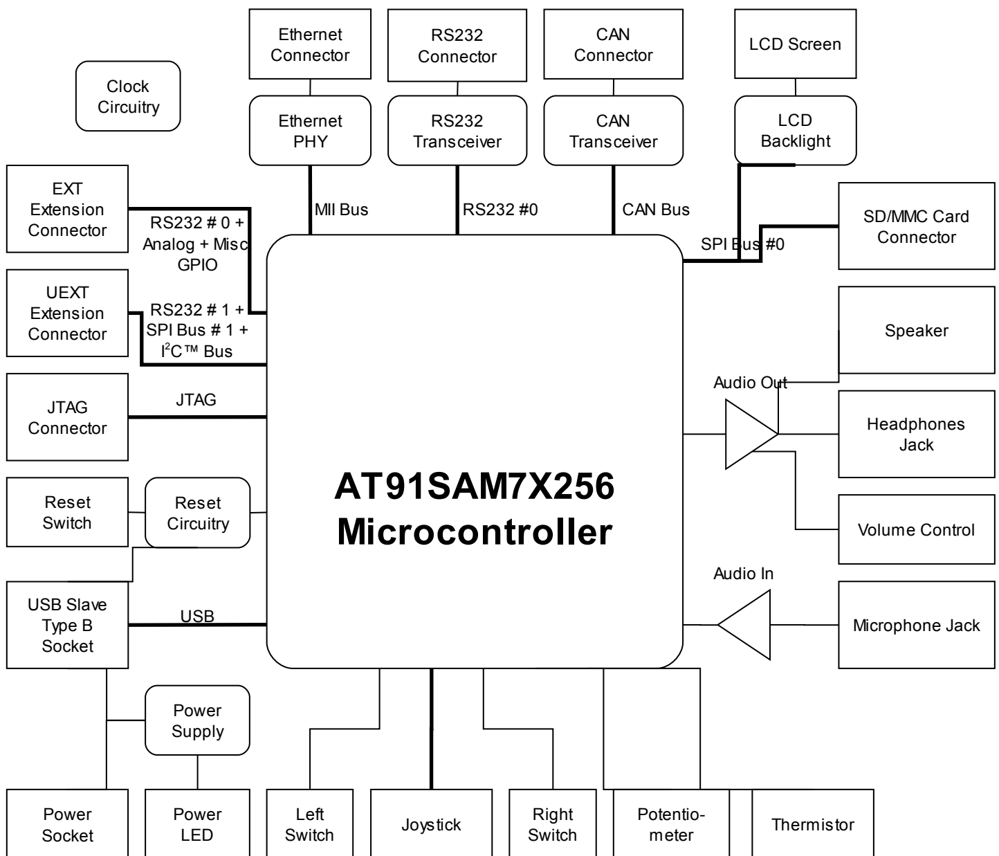
Figure 3-1- SAM7-EX256 Block Diagram
