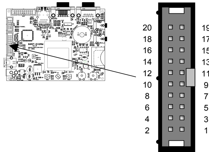
Figure 9-15 - JTAG Connector
