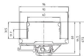
WEB closed housing
