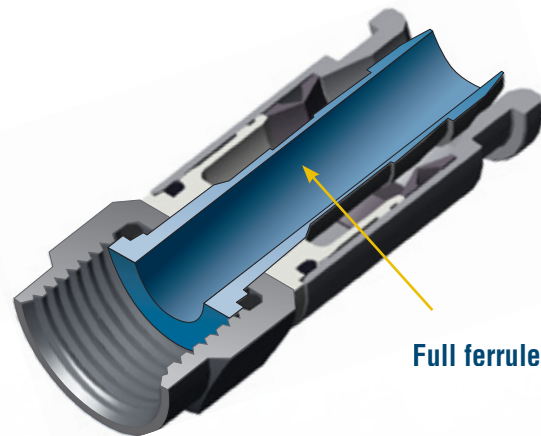
Full ferrule compression connector
