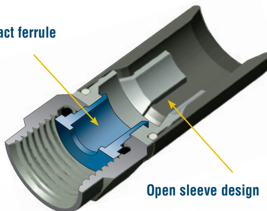
Klein Tools' Universal sleeve compact ferrule compression connector
