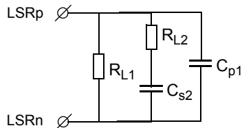
Figure 12: Load Circuit B Piezo Loudspeaker
