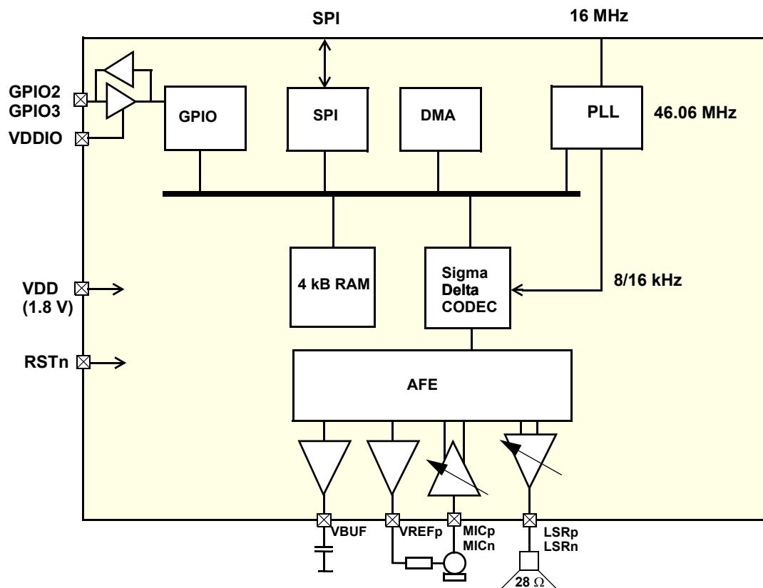
Figure 8: CODEC with AFE Block Diagram
