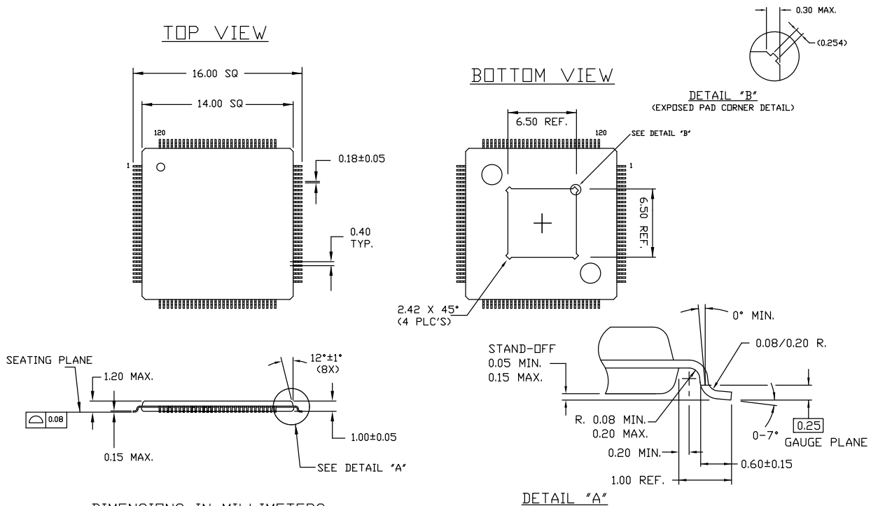
Figure 18. 120-pin TQFP (14 × 14 × 1.0 mm) AE120A (6.5 × 6.5 E-Pad) Package Outline, 001-48723
