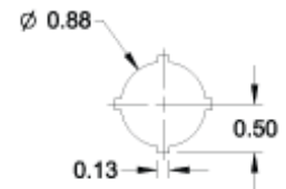
30.5mm Detail (1490 Series) 22.5mm Detail (1490M Series)
