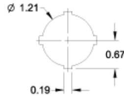
30.5mm Detail (1490 Series) 22.5mm Detail (1490M Series)
