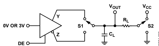
Figure 18. Driver Enable/Disable
