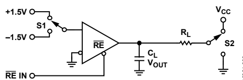
Figure 19. Receiver Enable/Disable
