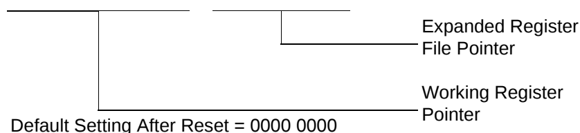
Figure 11. Register Pointer
