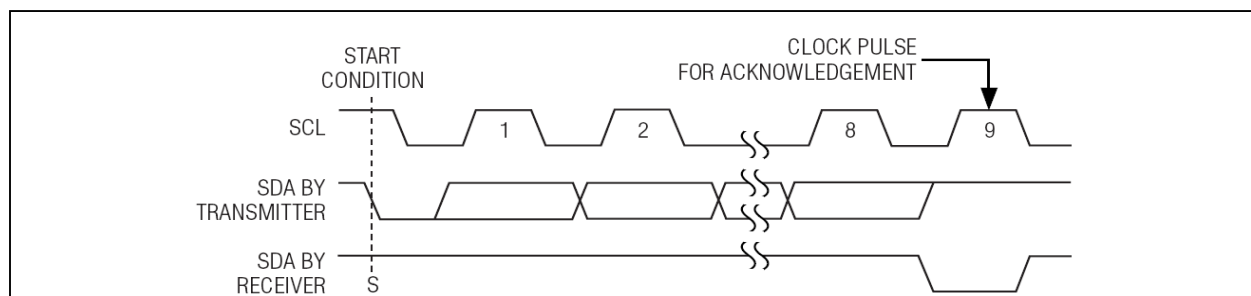
Figure 5 Acknowledge Signal
