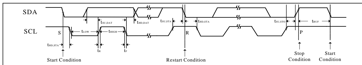
Figure 3 Interface Timing
