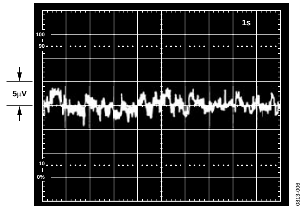
Figure 6. 0.1 Hz to 10 Hz Noise
