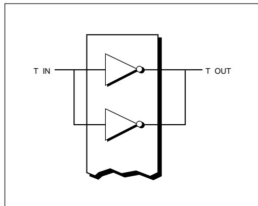
Figure 5. Parallel Drivers
