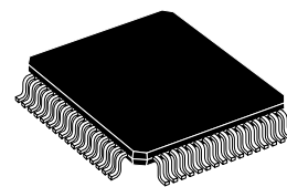
TQFP64 Full Plastic (10 x 10 x 1.40 mm)
