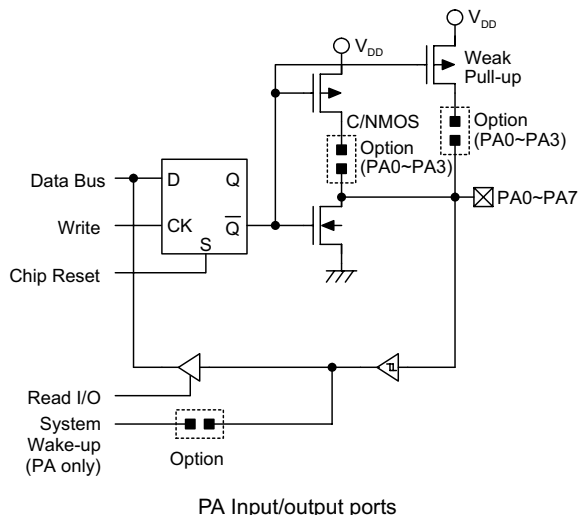
PA Input/output ports
