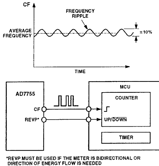
Figure 29. Interfacing the AD7755 to an MCU
