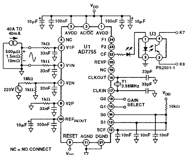
Figure 13. Test Circuit for Performance Curves
