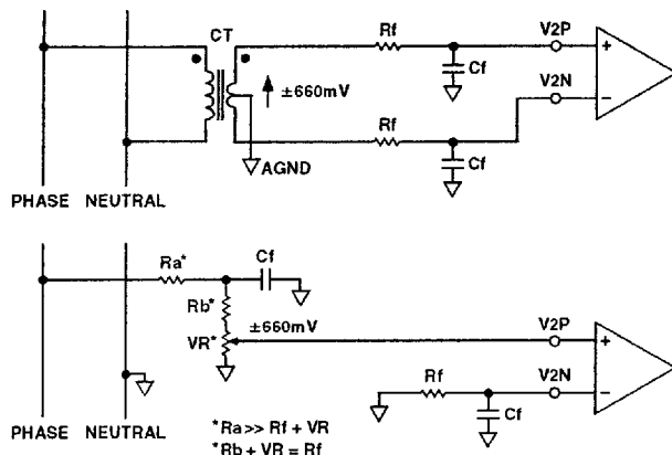
Figure 23. Typical Connections for Channel V2
