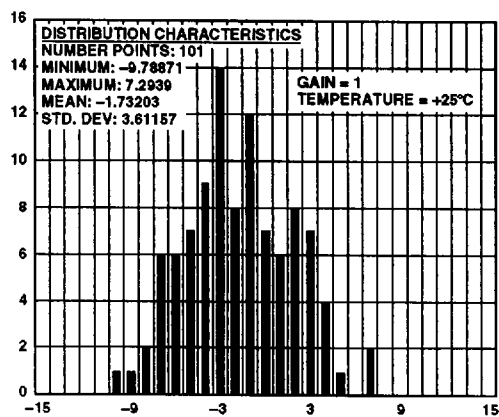
Figure 14. Channel 1 Offset Distribution (Gain = 1)
