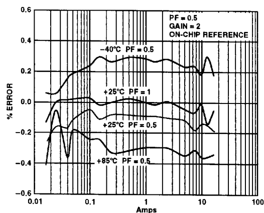
Figure 7. Error as a % of Reading (Gain = 2)
