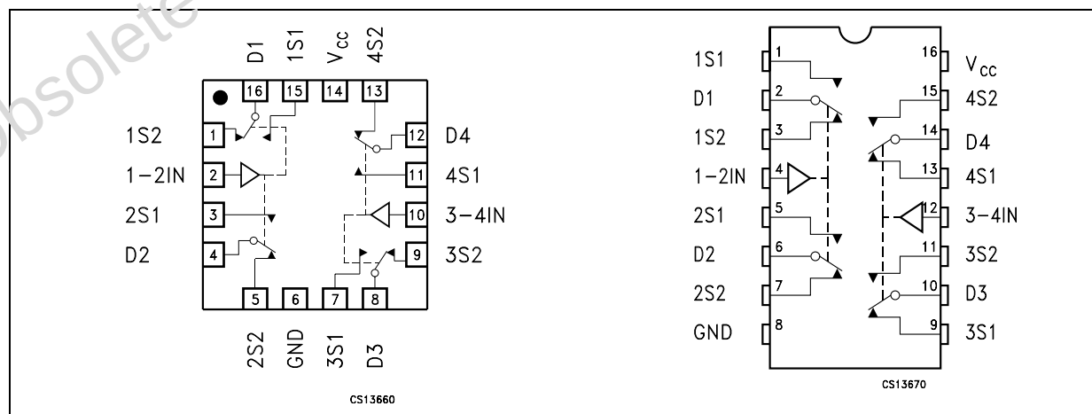
Figure 1: Pin Connection
