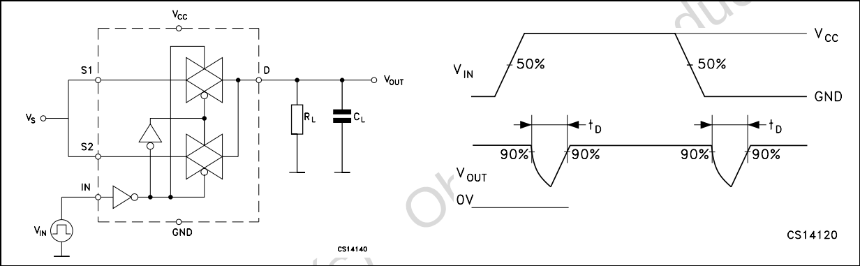
Figure 11: Switching Time And Charge Injection ( V_{GEN}=0\text{V} , R_{GEN}=0\Omega , R_L=1\text{M}\Omega , C_L=100\text{pF} )
