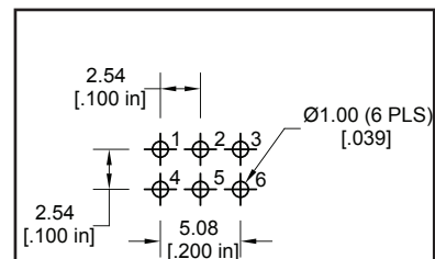
DOUBLE POLE PCB LAYOUT
