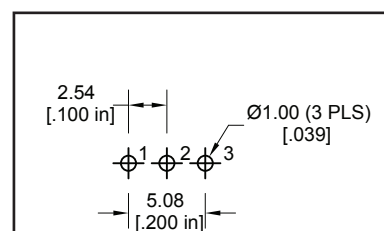
SINGLE POLE PCB LAYOUT
