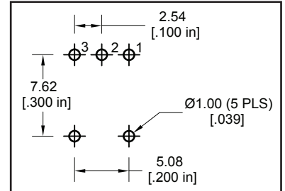
SINGLE POLE PCB LAYOUT
