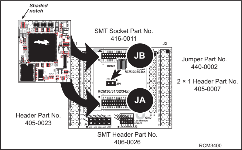
Figure 1. Top Side
