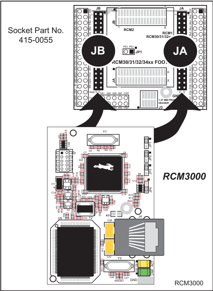
Figure 1. Top Side
