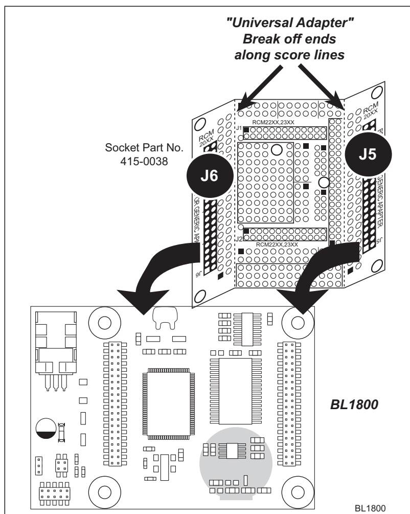
Figure 1. Top Side
