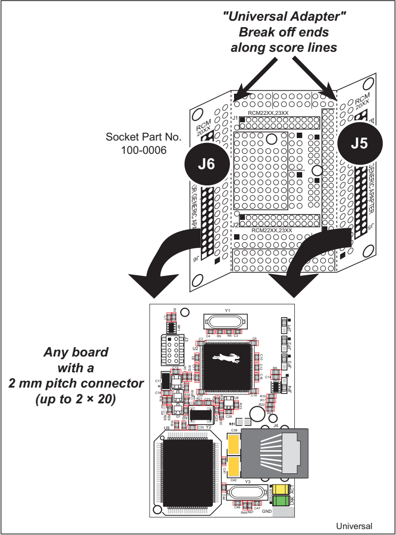
Figure 1. Top Side
