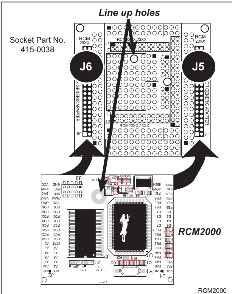
Figure 1. Top Side
