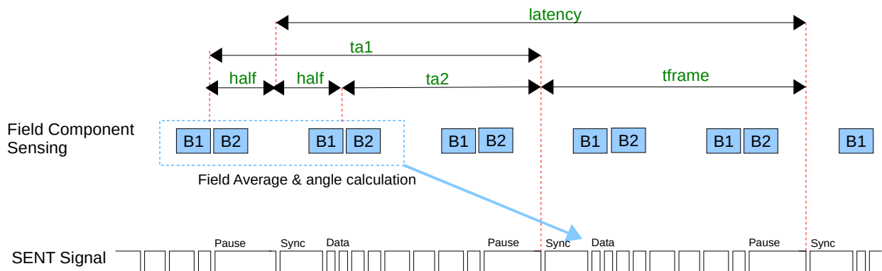
Figure 4: Latencies (acquisition to output delays) – FILTER = 1 (recommended)
