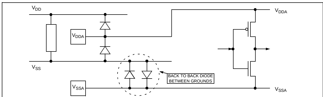
Figure 77. Multisupply Configuration
