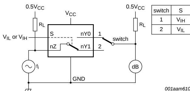
Fig 18. Test circuit for measuring isolation (OFF-state)
