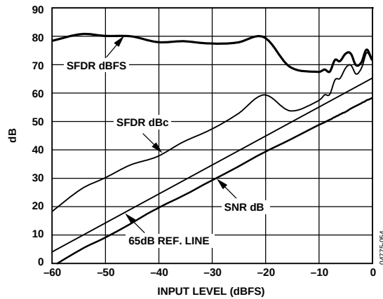
Figure 17. SFDR vs. Analog Input Level, A_{IN} = 70 \text{ MHz} , f_s = 65 \text{ MSPS} (–65 Grade)
