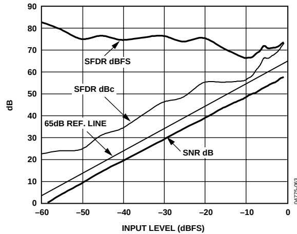
Figure 16. SFDR vs. Analog Input Level, A_{IN} = 70 \text{ MHz} , f_s = 80 \text{ MSPS} (–80 Grade)
