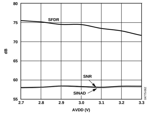
Figure 32. SNR, SINAD, SFDR vs. AVDD, A_{IN} = 70 MHz at -0.5 dBFS, 80 MSPS (-80 Grade)
