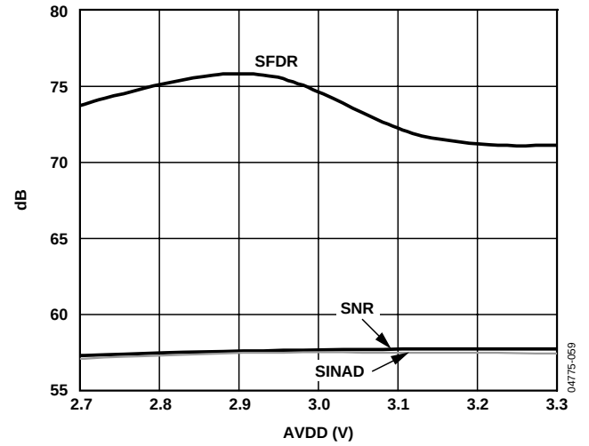
Figure 31. SNR, SINAD, SFDR vs. AVDD, A_{IN} = 70 MHz at -0.5 dBFS, 105 MSPS (-105 Grade)
