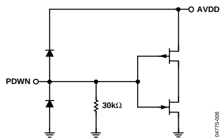
Figure 39. Power-Down Input
