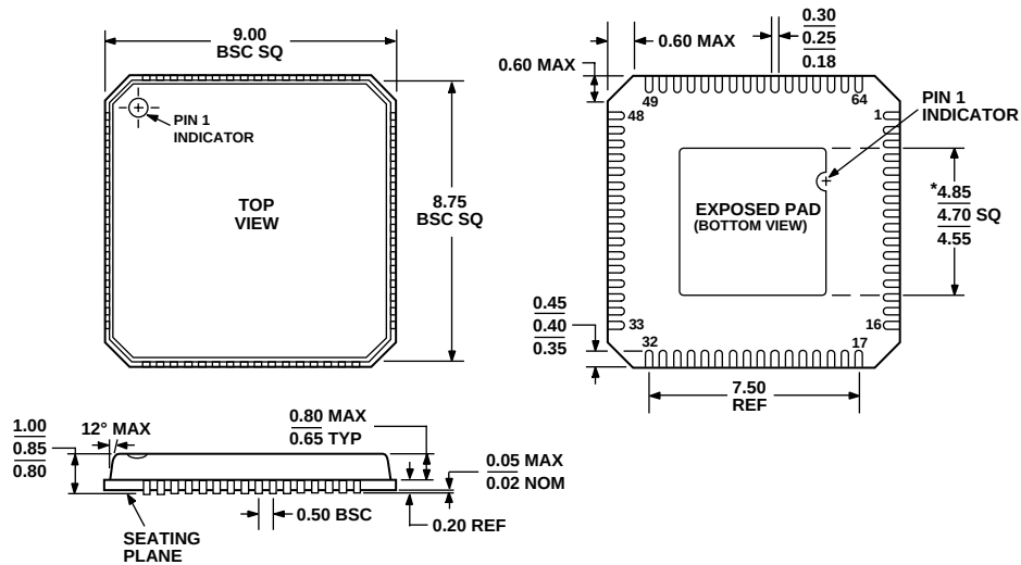
Figure 61. 64-Lead Lead Frame Chip Scale Package [LFCSP_VQ] 9 x 9 mm Body, Very Thin Quad (CP-64-1) Dimensions shown in millimeters
