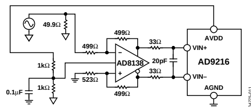
Figure 44. Driving the ADC with the AD8138
