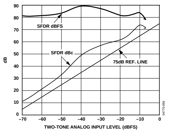
Figure 21. Two-Tone IMD Performance vs. Input Drive Level (69.1 MHz and 70.1 MHz; f_s = 65 \text{ MSPS} (–65 Grade); F_1, F_2 Levels Equal)
