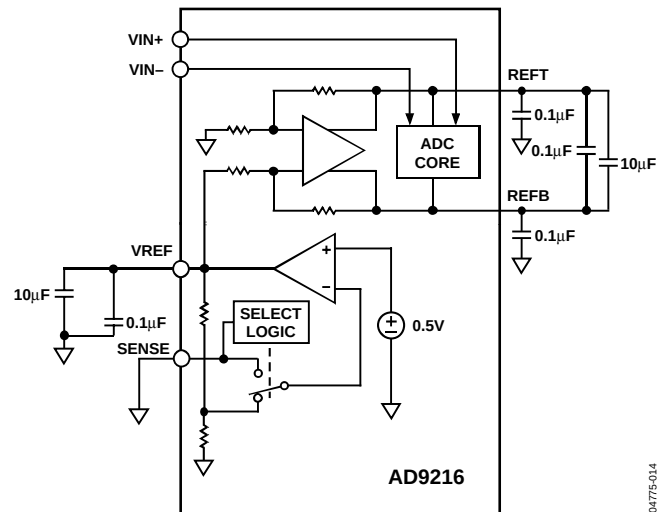
Figure 47. Internal Reference Configuration (One Channel Shown)
