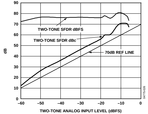
Figure 19. Two-Tone IMD Performance vs. Input Drive Level (69.1 MHz and 70.1 MHz; f_s = 105 \text{ MSPS} (–105 Grade); F_1, F_2 Levels Equal)
