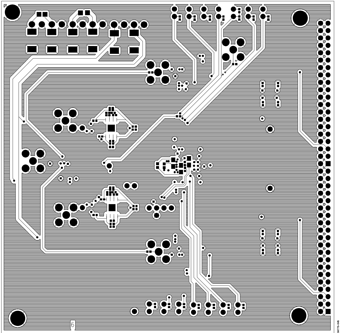
Figure 58. PCB Bottom-Side Copper Routing
