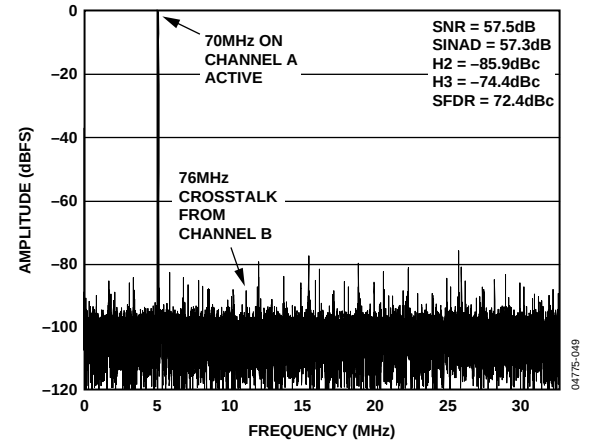
Figure 9: FFT: f_s = 65 MSPS, A_{IN} = 70 MHz, 76 MHz ( -65 Grade) (A Port FFT while Both A and B Ports Are Driven at -0.5 dBFS)
