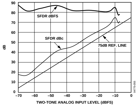
Figure 20. Two-Tone IMD Performance vs. Input Drive Level (69.1 MHz and 70.1 MHz; f_s = 80 \text{ MSPS} (–80 Grade); F_1, F_2 Levels Equal)
