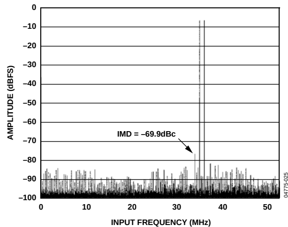
Figure 18. Two-Tone IMD Performance F_1, F_2 = 69.1 \text{ MHz}, 70.1 \text{ MHz} at –7 dBFS, 105 \text{ MSPS} (–105 Grade)
