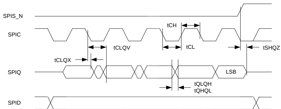
Figure 21. SPI Output Timing
