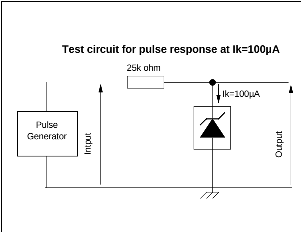
Figure 7. Test circuit for pulse response at I_k=100\mu A
