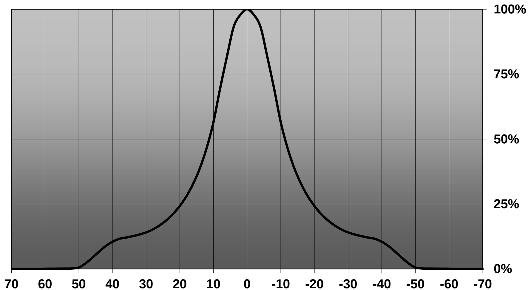
Relative intensity of C12095_MINNIE-M (Luxeon M)
