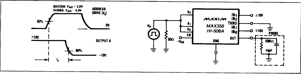
Figure 1. Access Time vs. Logic Level (High)
