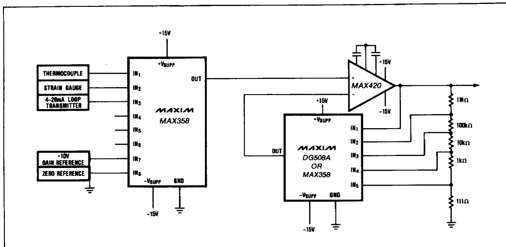
Figure 7. Typical Data Acquisition Front End
