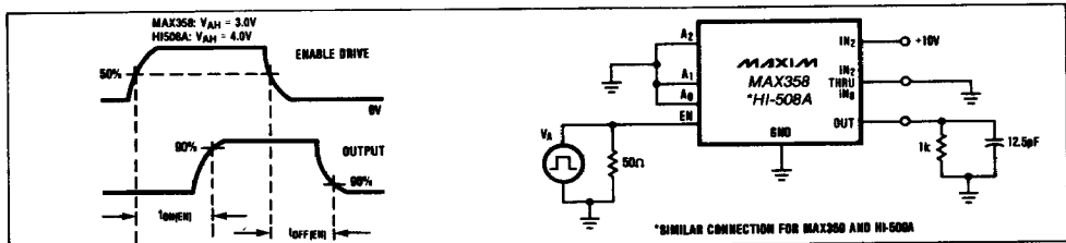
Figure 3. Enable Delay ( t_{ONEN} , t_{OFFEN} )
