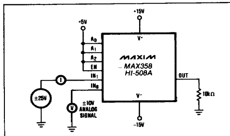
Figure 5. Input Leakage Current (Overvoltage)
