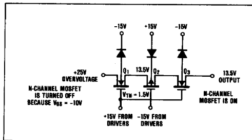
Figure 11. +25\text{V} Overvoltage Input to the ON Channel
