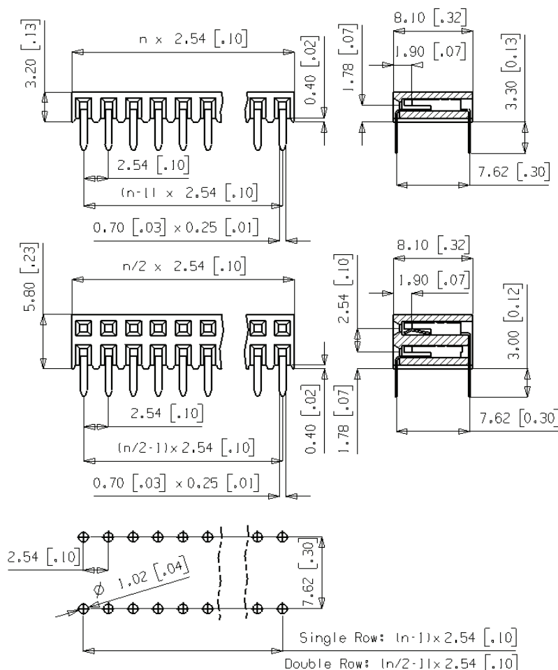
PCB Layout
