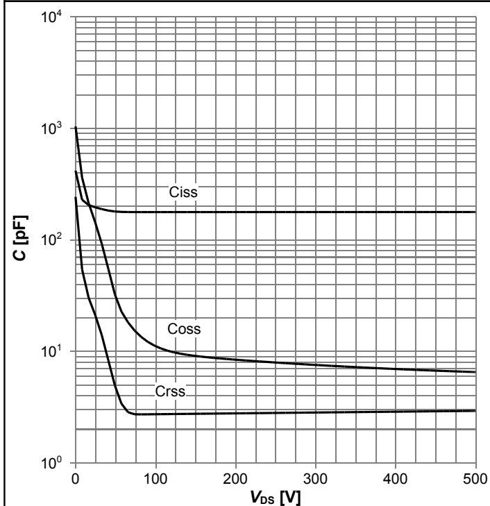
Diagram 13: Typ. capacitances
