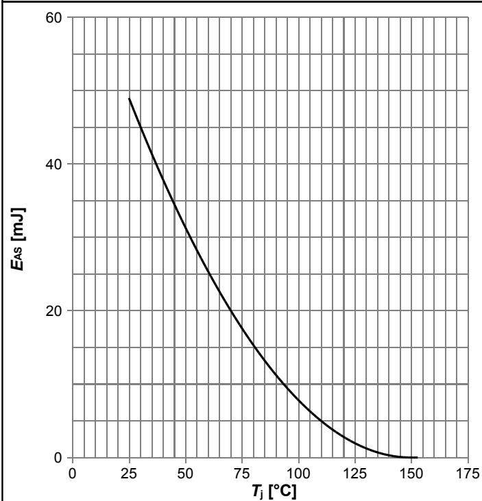
Diagram 11: Avalanche energy
