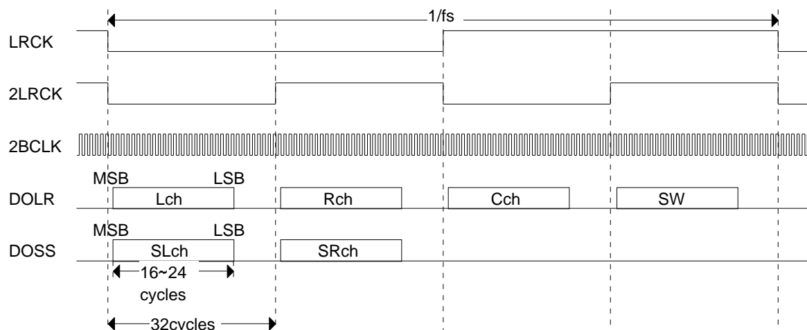
Figure 5.10 I²S Format Interface Between M65863FP and DAC(dacform[0]=1)
