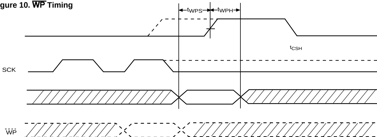
Figure 10. WP Timing
