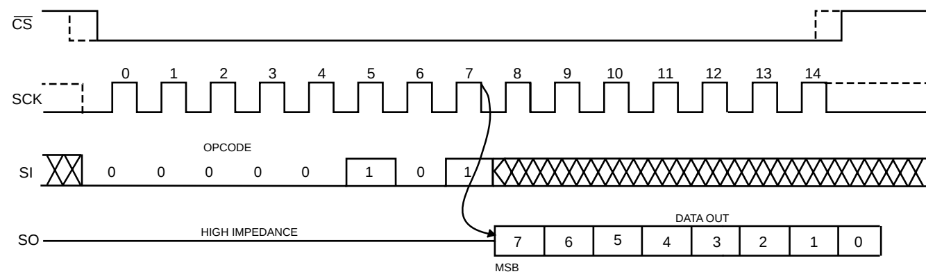
Figure 5. RDSR Timing
