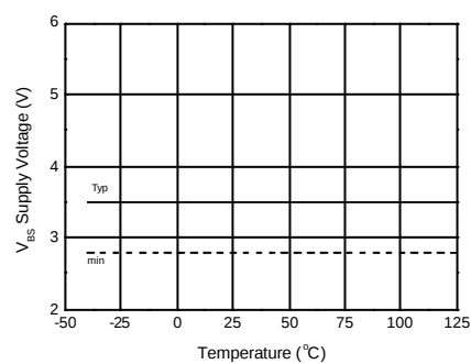
Figure 25b. VBS UnderVoltage Threshold(-) vs Temperature
