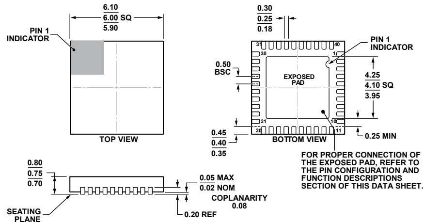
Figure 42. 40-Lead Lead Frame Chip Scale Package [LFCSP_WQ] 6 mm × 6 mm Body, Very Very Thin Quad (CP-40-9) Dimensions shown in millimeters
