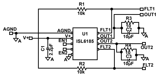
FIGURE 32A. ISL6185xEVAL SCHEMATIC
