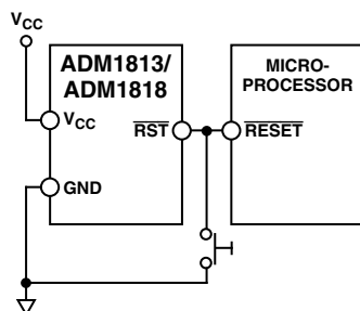
Figure 3. ADM1813/ADM1818 Typical Application
