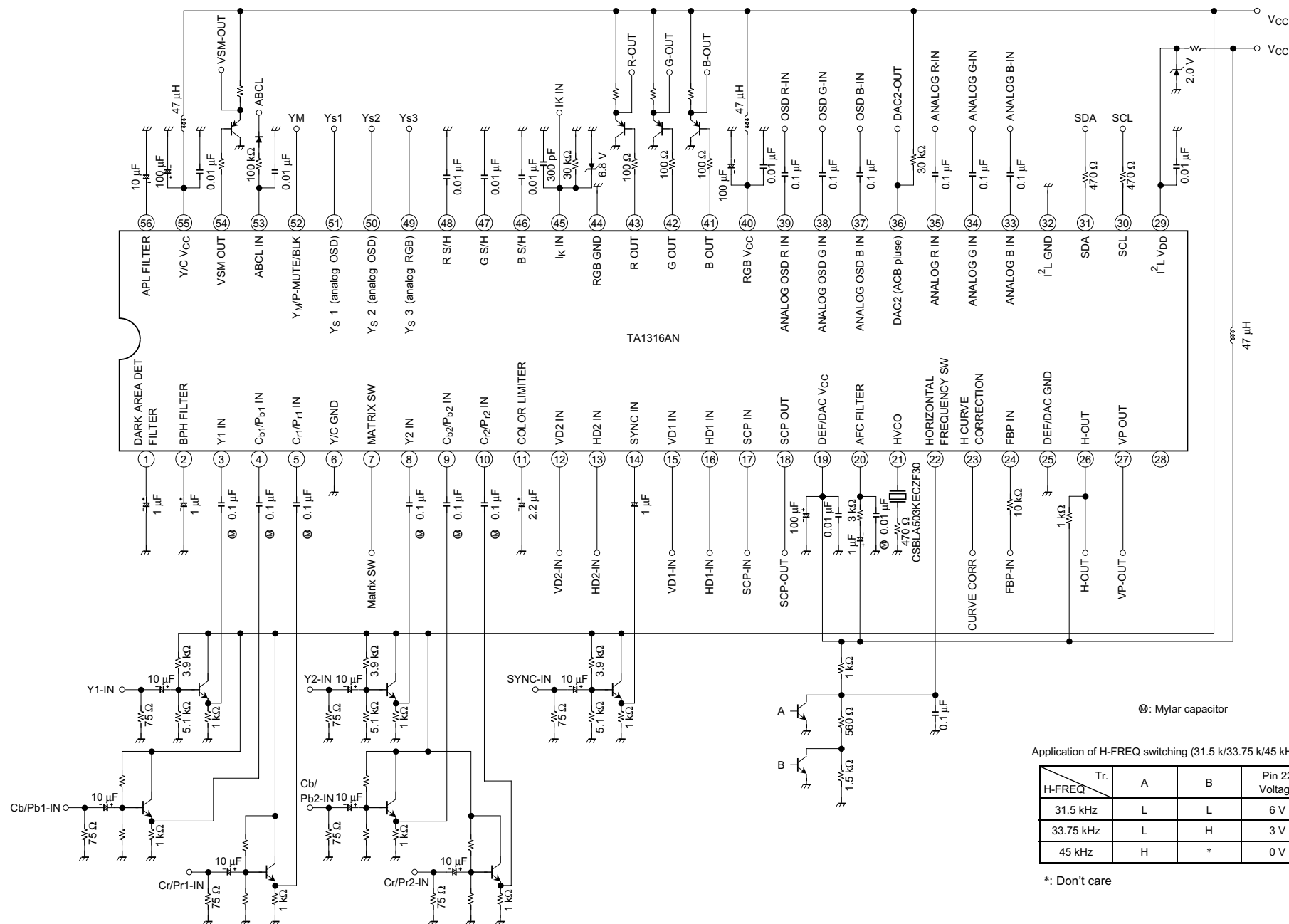
Application Circuit
