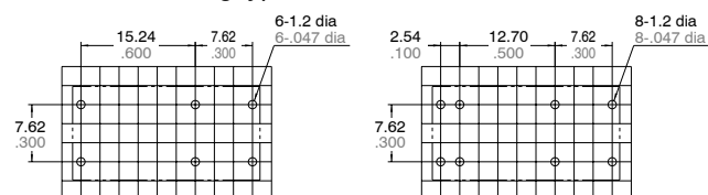
PC board pattern (Bottom view) Single side stable 2 coil latching type 1 coil latching type
