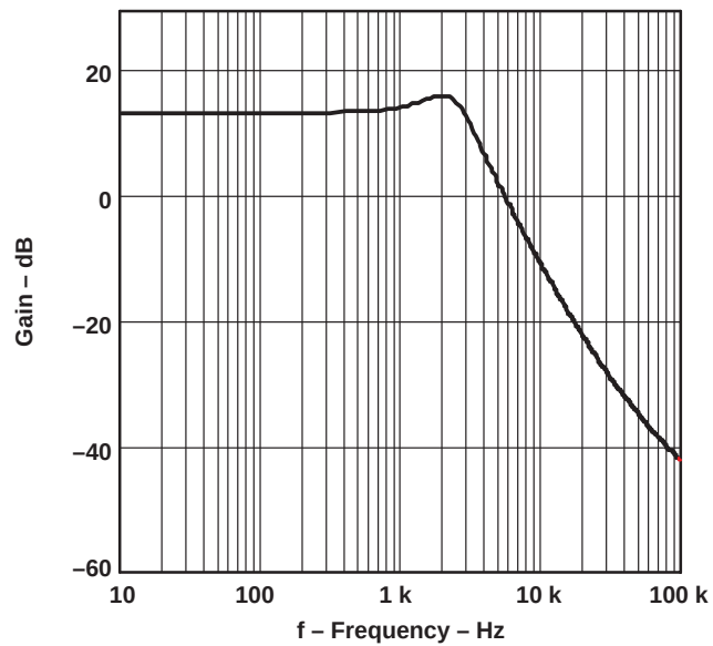
Figure 2–1. Power Stage Gain
