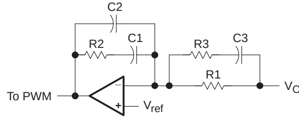
Figure 2–3. Compensation Circuit
