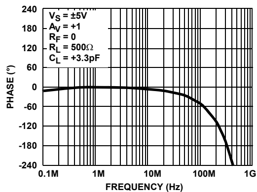
FIGURE 2. PHASE vs FREQUENCY
