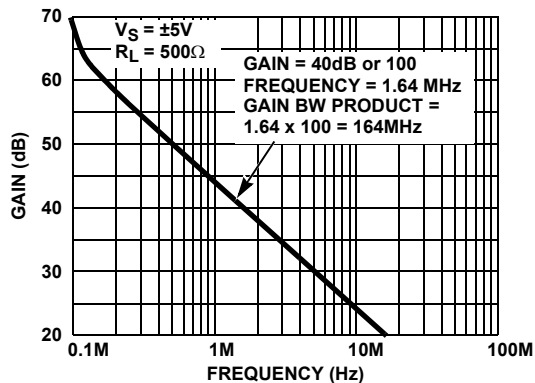
FIGURE 4. GAIN BANDWIDTH PRODUCT
