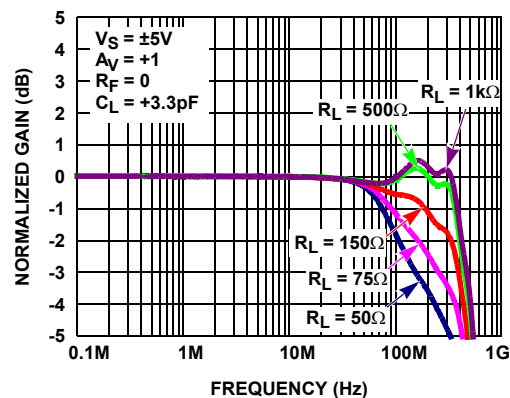
FIGURE 8. GAIN vs FREQUENCY FOR VARIOUS R_{LOAD} ( A_V = +1 )
