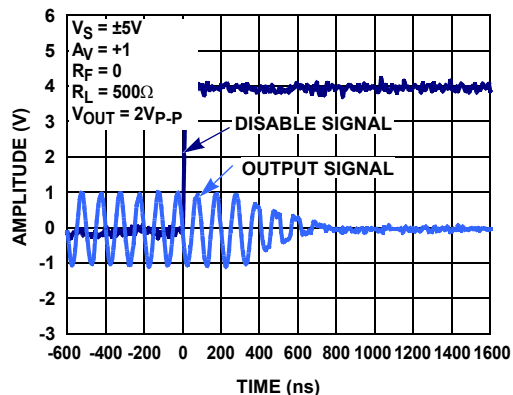
FIGURE 30. TURN-OFF TIME
