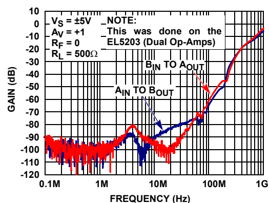
FIGURE 26. CHANNEL-TO-CHANNEL ISOLATION
