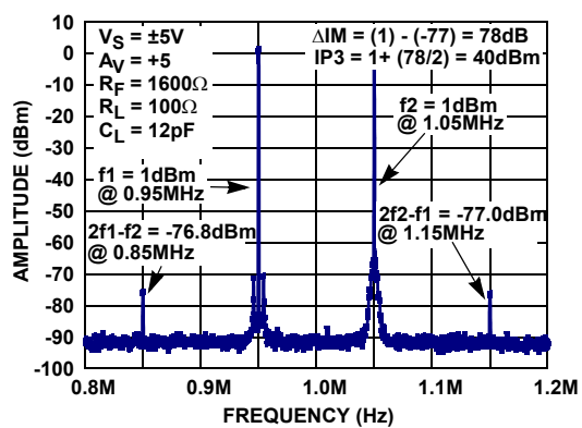
FIGURE 35. THIRD ORDER IMD INTERCEPT (IP3)
