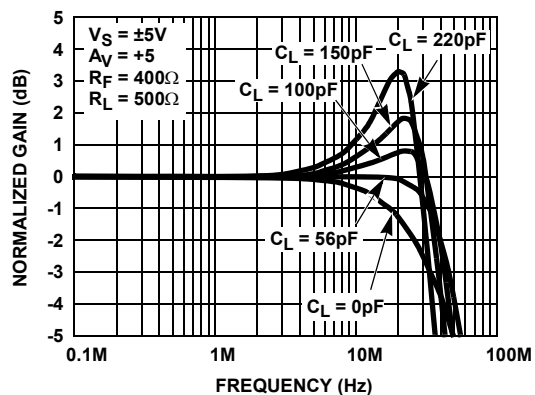
FIGURE 13. GAIN vs FREQUENCY FOR VARIOUS C_{LOAD} ( A_V = +5 )
