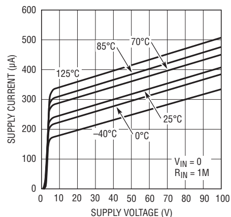
LTC6101HV: Supply Current vs Supply Voltage
