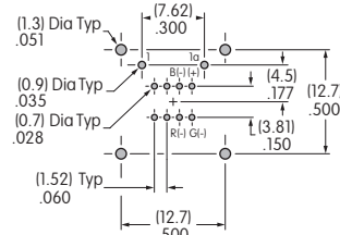
Terminal Detail
