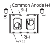
Terminal Detail
