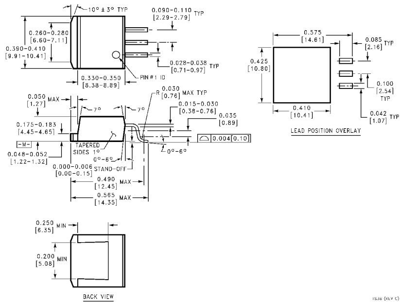
TO-263 Surface-Mount Package (S) Order Number LM7805S or LM7812S NS Package Number TS3B
