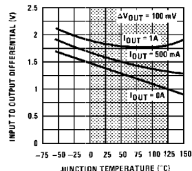
Dropout Voltage
