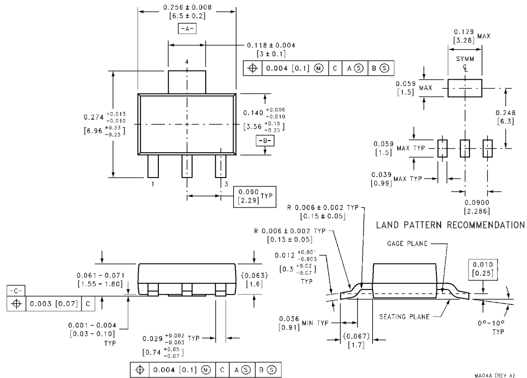
3-Lead SOT-223 Package Order Part Number LM340MP-5.0 NS Package Number MA04A
