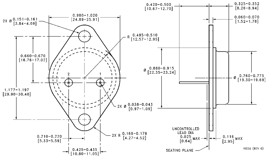
TO-3 Metal Can Package (K) Order Number LM340AK-5.0, LM140K-5.0, LM340K-5.0, LM140K-12, LM340K-12, LM140K-15, LM340K-15, LM7806CK, LM7808CK, LM7818CK or LM7824CK NS Package Number K02A
