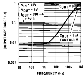
Output Impedance
