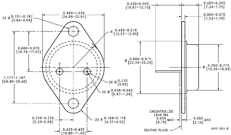
TO-3 Metal Can Package (K) Mil-Aero Products Order Number LM140AK-5.0/883, LM140K-5.0/883, LM140AK-12/883, LM140K-12/883, LM140AK-15/883 or LM140K-15/883 NS Package Number K02C
