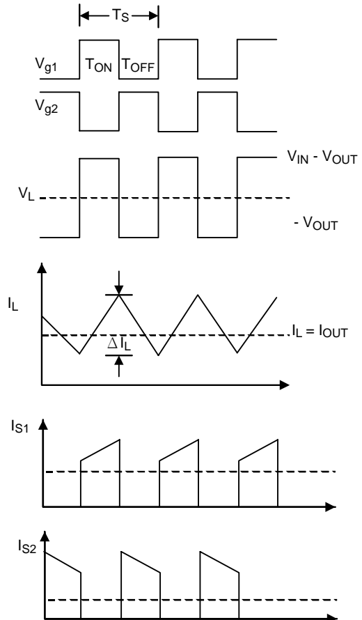
Figure 8. The waveforms of synchronous step-down converter
