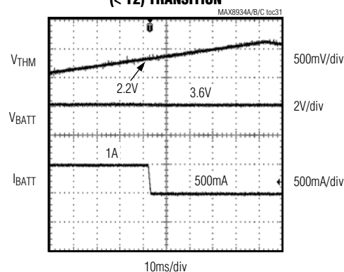
THM NORMAL TO THM COLD (< T2) TRANSITION
