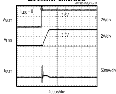
LDO STARTUP WAVEFORMS
