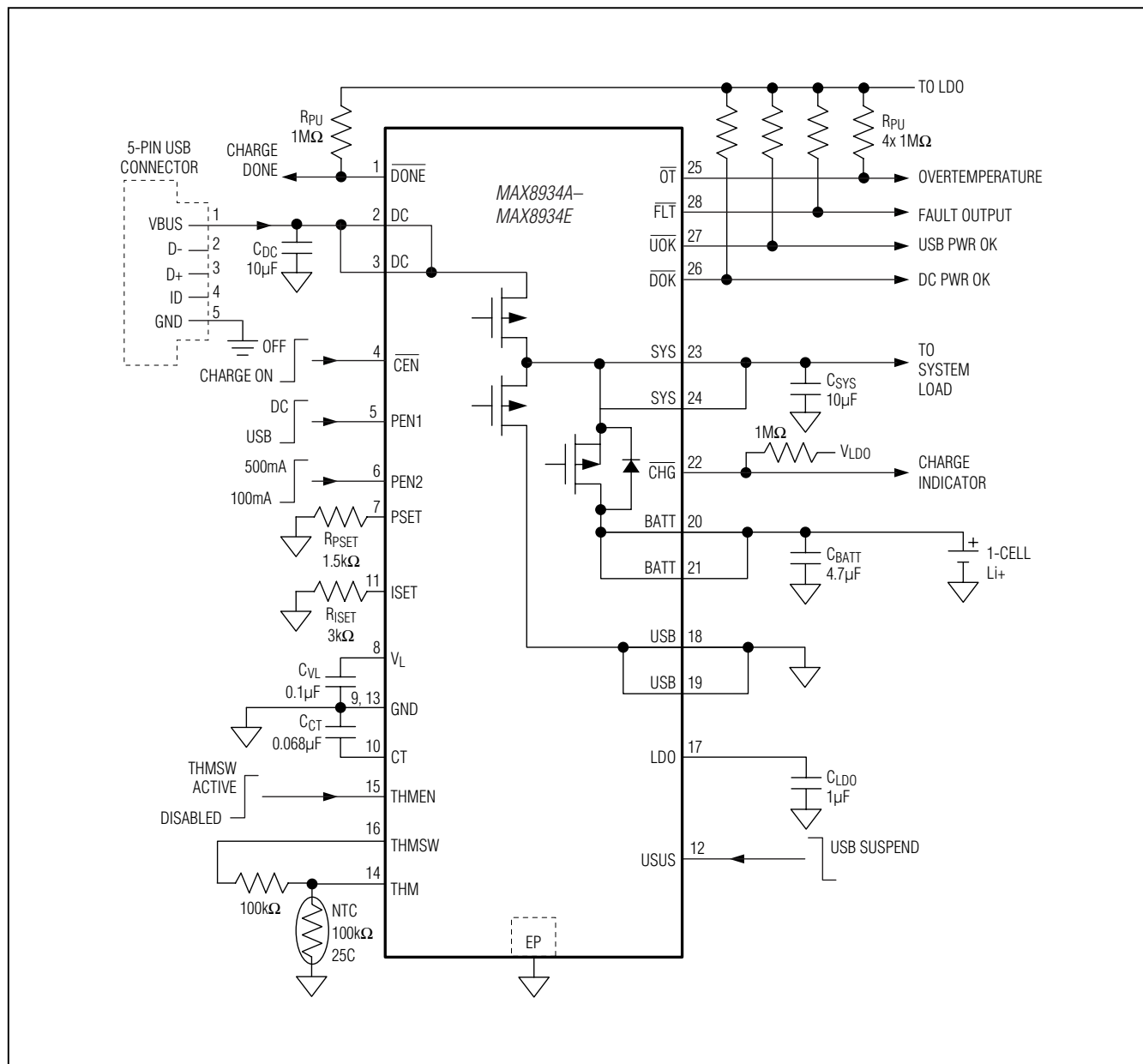
Figure 3. Typical Application Circuit Using a 5-Pin USB Connector or Other DC/USB Common Connector
