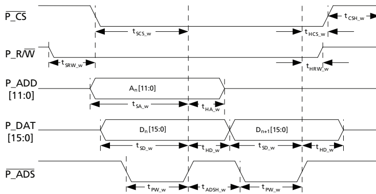
Figure 4-7: External Timing for Auto-Increment Write Cycle
