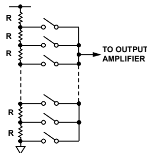
Figure 25. Resistor String
