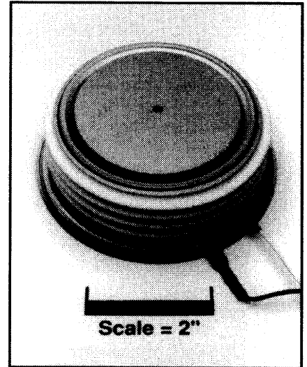
C784 Phase Control SCR 1650 Amperes Average, 4500 Volts
