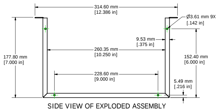
SIDE VIEW OF EXPLODED ASSEMBLY
