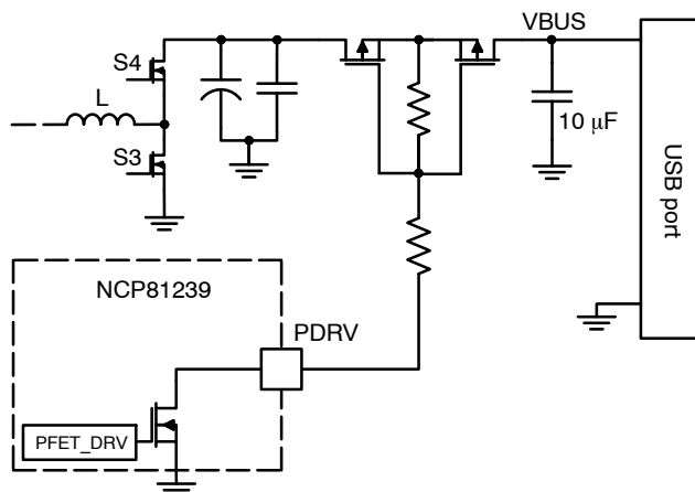
Figure 12. PFET Drive
