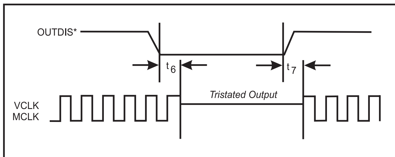
Tristated Timing
