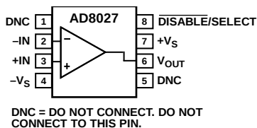
Figure 1. 8-Lead SOIC, AD8027
