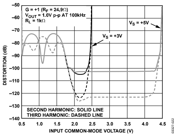
Figure 27. Harmonic Distortion vs. Input Common-Mode Voltage, \overline{\text{DISABLE/SELECT}} = \text{High}
