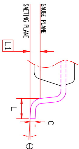
DETAIL A
